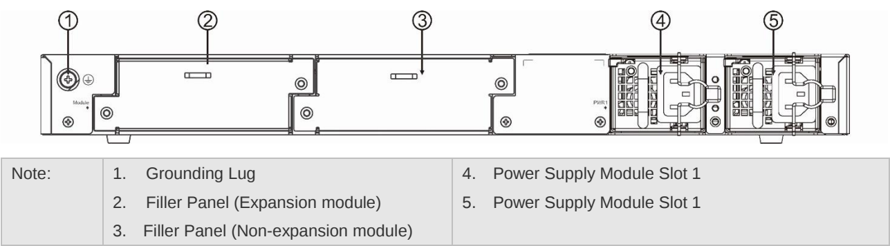
Figure 1-13 Rear Panel of RG-CS85-24SFP/8GT8XS-D
