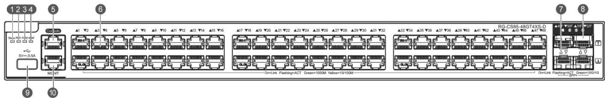
Figure 1-7 Front Panel of RG-CS85-48GT4XS-D
