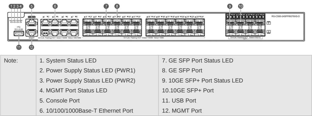
Figure 1-12 Front Panel of RG-CS85-24SFP/8GT8XS-D
