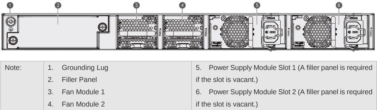
Figure 1-18 Rear Panel of RG-CS85-48GT4XS-HPD
