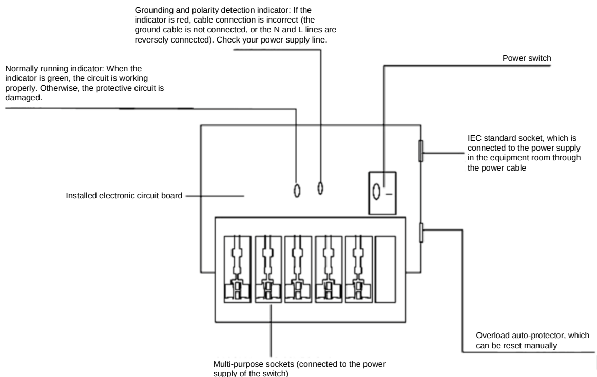
Figure C-1 Power Arrester
