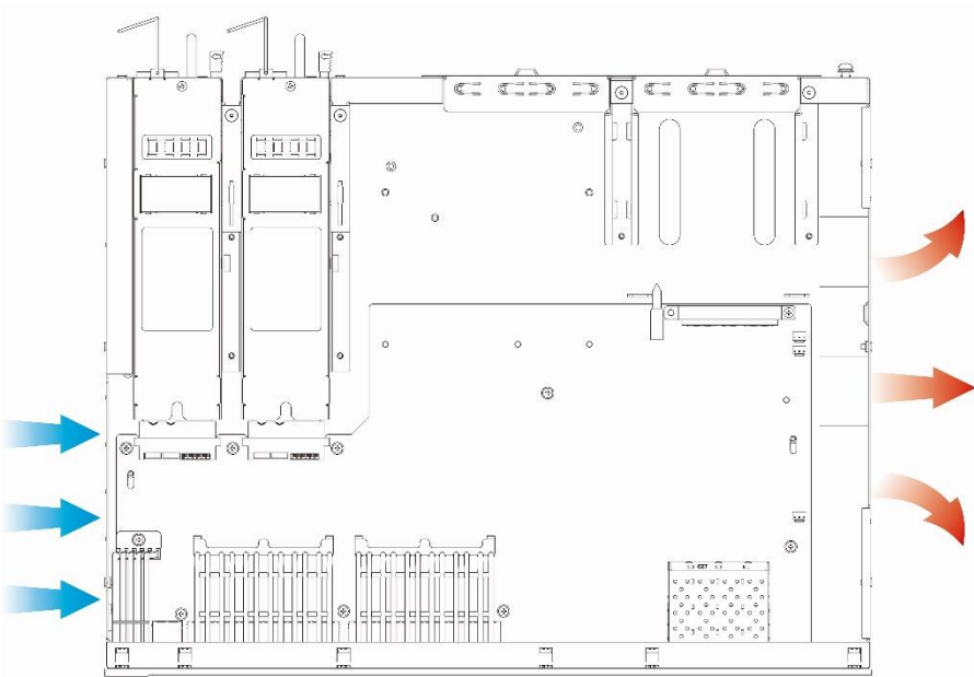
Figure 1-4 Airflow Direction
