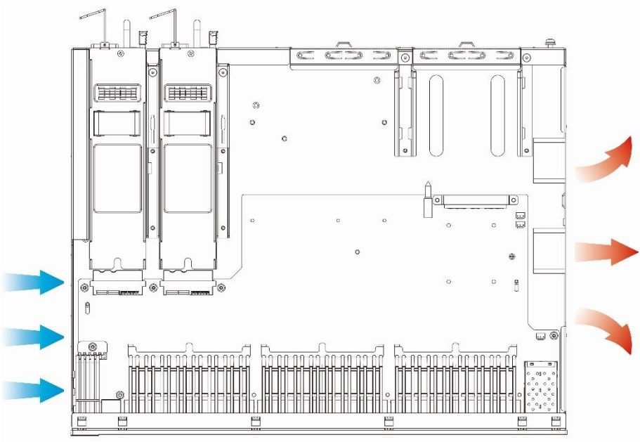
Figure 1-10 Airflow Direction
