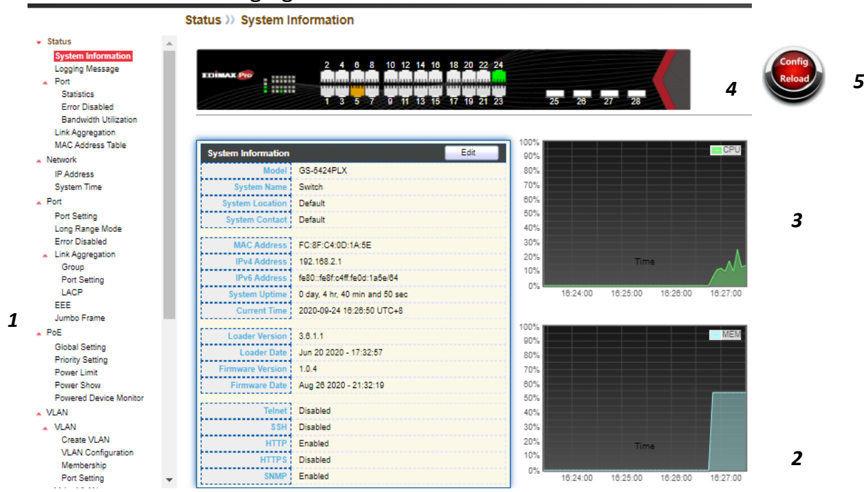
Figure 11 - User Interface
