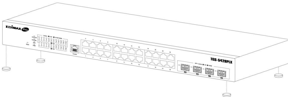
Figure 4 - Desktop Installation
