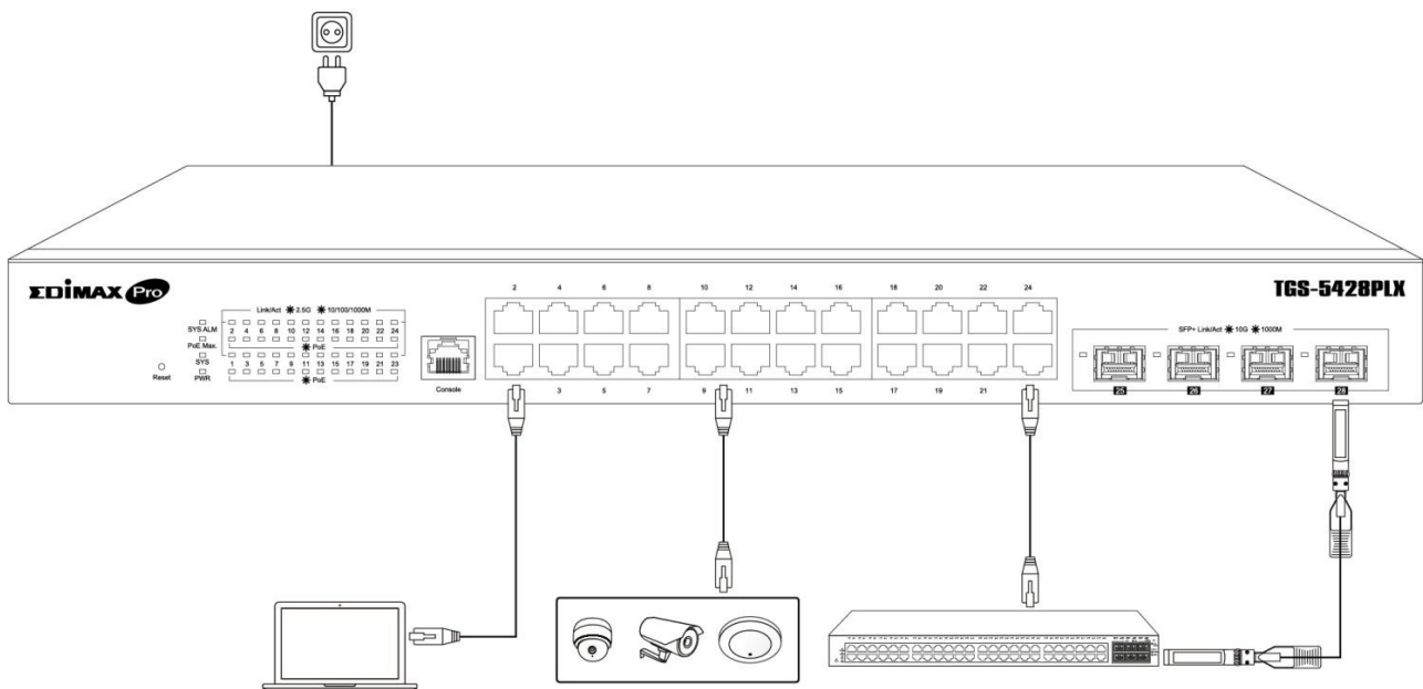
Figure 8 - PC Connect
