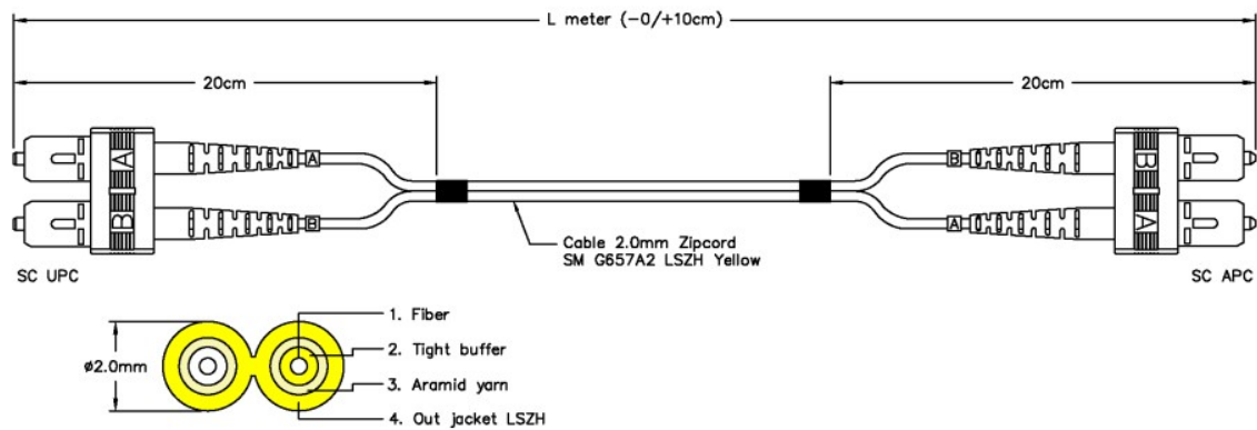
LinkIT FiberPatch SM G657A2 SC-SC/APC Yellow
