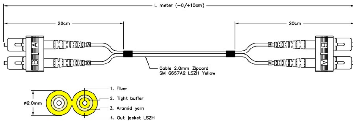
LinkIT FiberPatch SM G657A2 SC/SC Yellow
