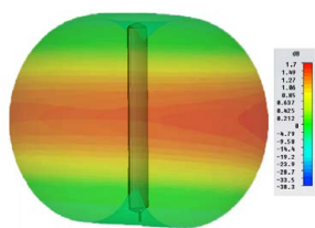
3D Plot (850MHz)
