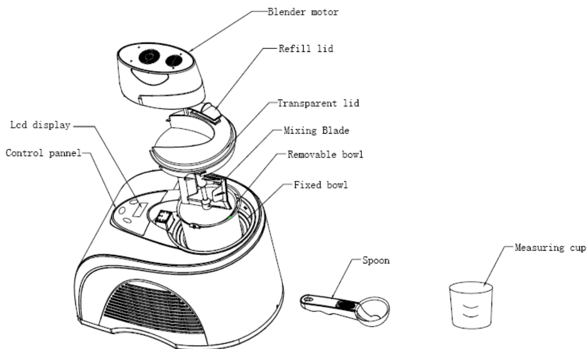
Illustration 1-Exploded View
