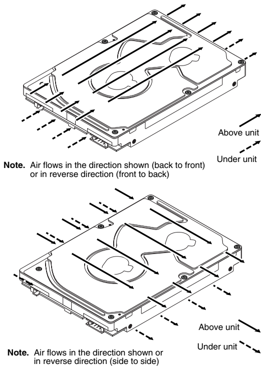
Figure 7. Air flow
