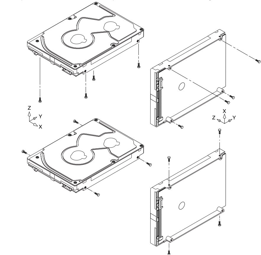
Figure 3. Recommended mounting
