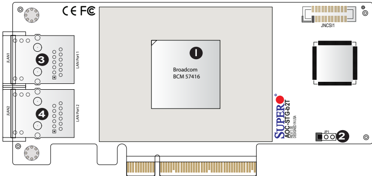
The AOC-STG-b2T Layout
