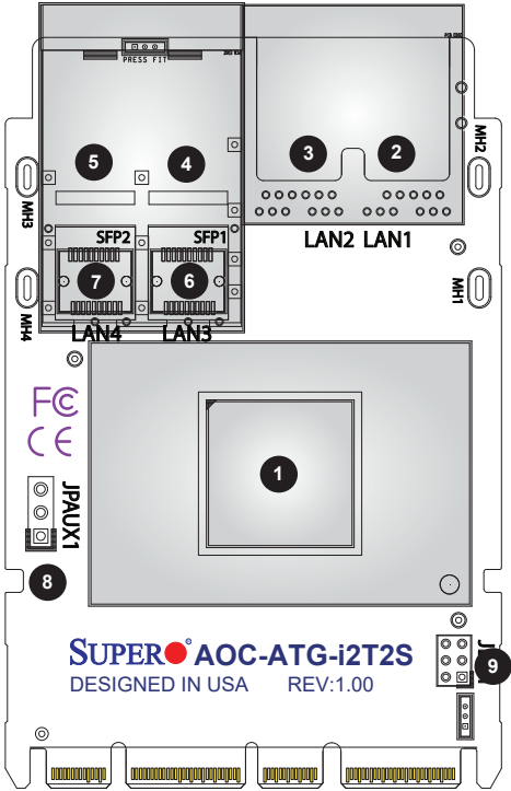
AOC-ATG-i2T2SM Layout
