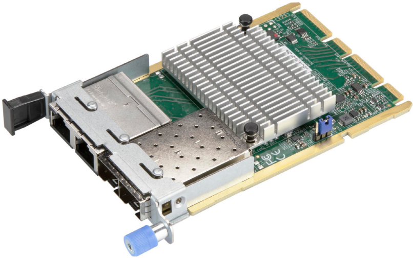
AOC-ATG-i2T2SM Image
