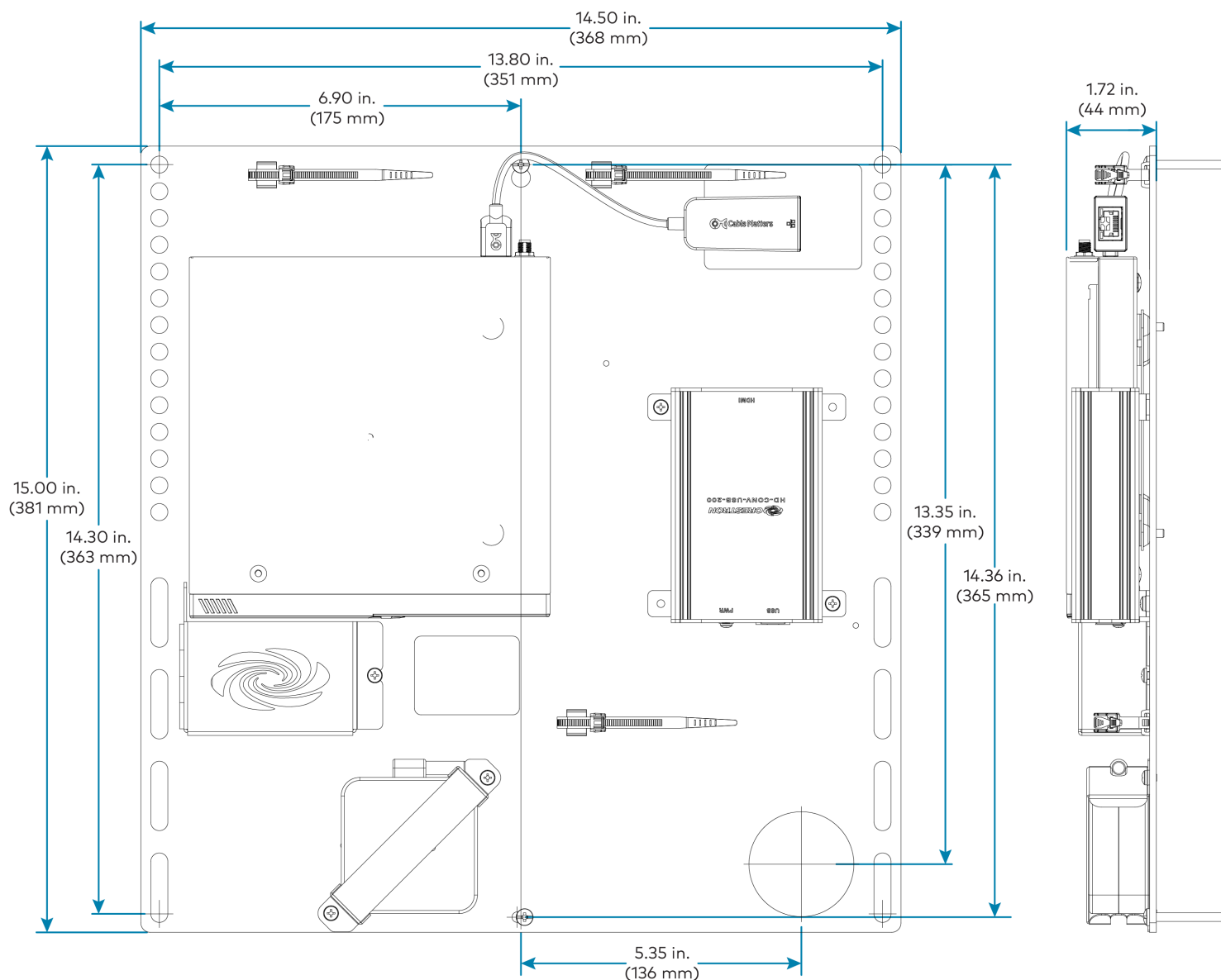
UC Bracket Assembly (UC-BRKT-200-S-T-ASSY)
